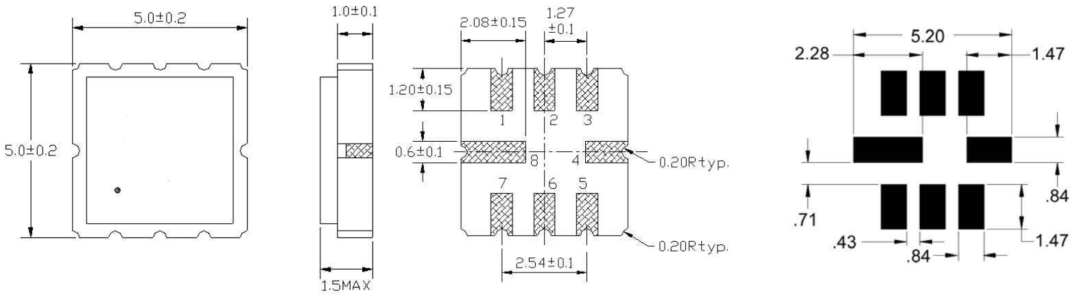
Figure 2) Land Pattern
