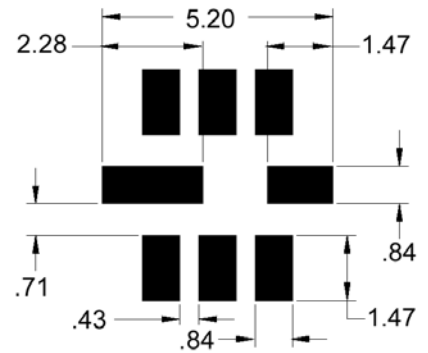
Figure 2) Land Pattern
